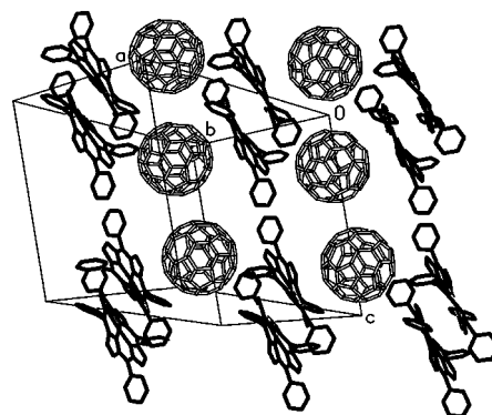
Figure 5. Molecular packing in [Cu(tp)]_2 \cdot C_{60} ( 8 ), projection on the plane (1–10).
