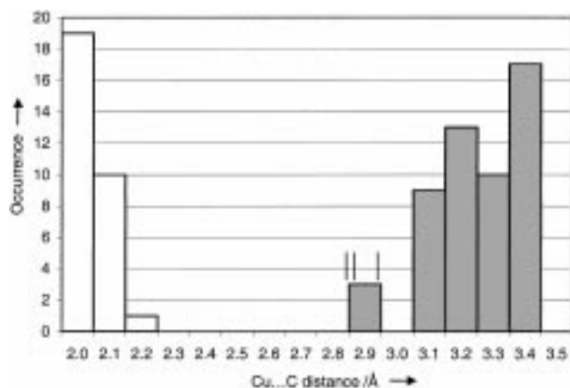
Figure 12. Histogramm of bonding (white columns) and nonvalent (grey) Cu \cdots C (olefin) distances from CSD data. Secondary bonding distances in 10 are shown as thin lines.
