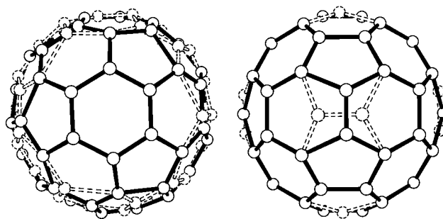
Figure 4. Rotational disorder of a C_{60} molecule (one hemisphere is shown). Left: in 2 , a 60° rotation around the threefold axis. Right: in 8 , a 180° rotation around the axis through the midpoint of 5/6 edges.
