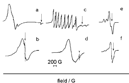
Figure 7. The ESR spectra of a) [Mn(tp)], b) 4 , c) [Co(tp)], d) 6 , e) [Cu(tp)] and f) 9 at 77 K in argon atmosphere. Arrows show the position of g = 2.0022 .
