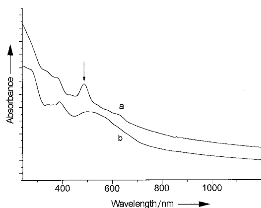
Figure 9. The UV-visible spectra of a) 4 and b) \text{C}_{70} in KBr matrix. The [\text{Mn}(\text{tpp})] absorption band is marked by an arrow.
