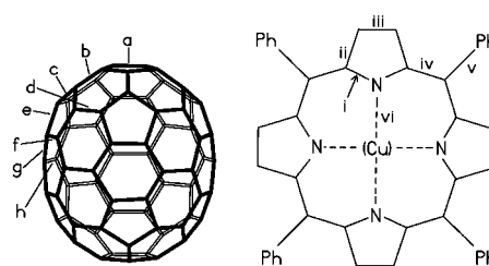
Scheme 1. Notation of chemically nonequivalent bonds in \text{C}_{70} and in \text{H}_2\text{TPP} or [\text{Cu}(\text{tpp})] .
