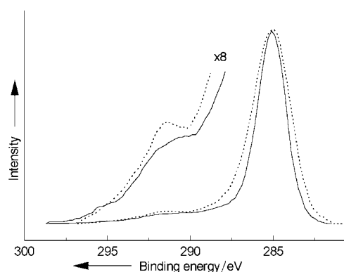
Figure 11. X-ray photoelectron C1s spectra of H 2 TPP (dashed) and 2 (solid line), and a portion thereof multiplied eight times.
