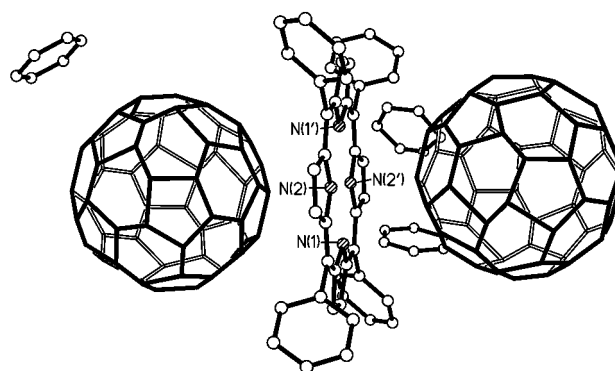
Figure 1. Molecules in the crystal of \text{H}_2\text{TPP} \cdot 2\text{C}_{60} \cdot 3\text{C}_6\text{H}_6 ( 1 ).
